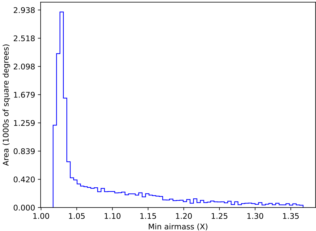
ddf_acor_sf20_lsf40_lsr50_v3.4_10yrs WFD r band: Min airmass
