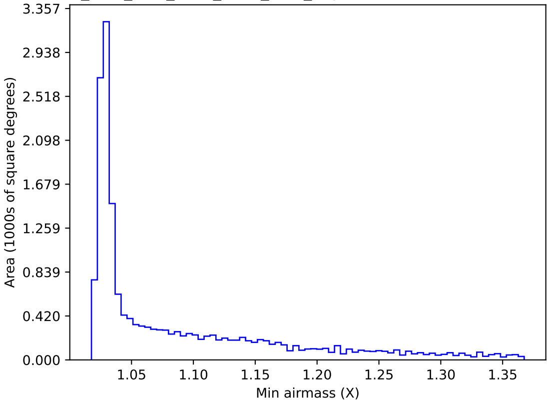
ddf_acor_sf20_lsf40_lsr50_v3.4_10yrs WFD i band: Min airmass
