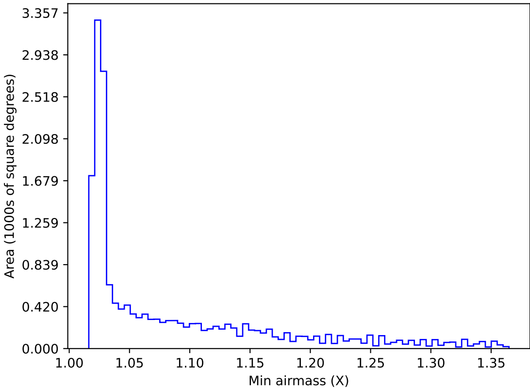
ddf_acor_sf20_lsf40_lsr50_v3.4_10yrs WFD all bands: Min airmass
