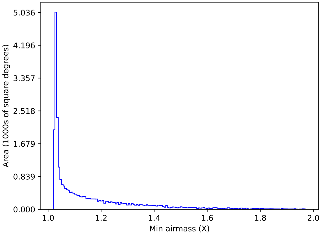
ddf_acor_sf20_lsf40_lsr50_v3.4_10yrs All sky z band: Min airmass
