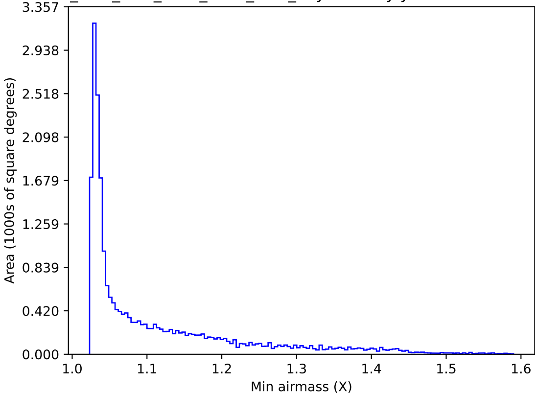
ddf_acor_sf20_lsf40_lsr50_v3.4_10yrs All sky y band: Min airmass
