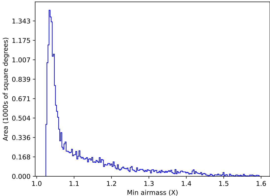
ddf_acor_sf20_lsf40_lsr50_v3.4_10yrs All sky u band: Min airmass
