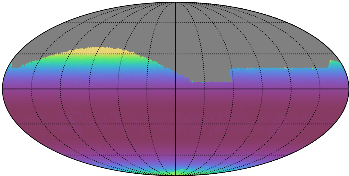
ddf_acor_sf20_lsf40_lsr50_v3.4_10yrs All sky r band: Min airmass
