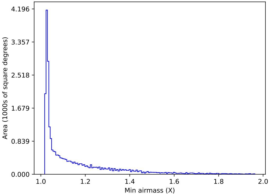
ddf_acor_sf20_lsf40_lsr50_v3.4_10yrs All sky r band: Min airmass
