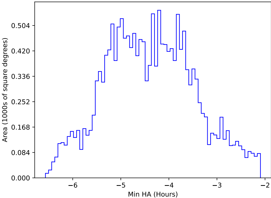
ddf_acor_sf20_lsf40_lsr50_v3.4_10yrs WFD z band: Min HA
