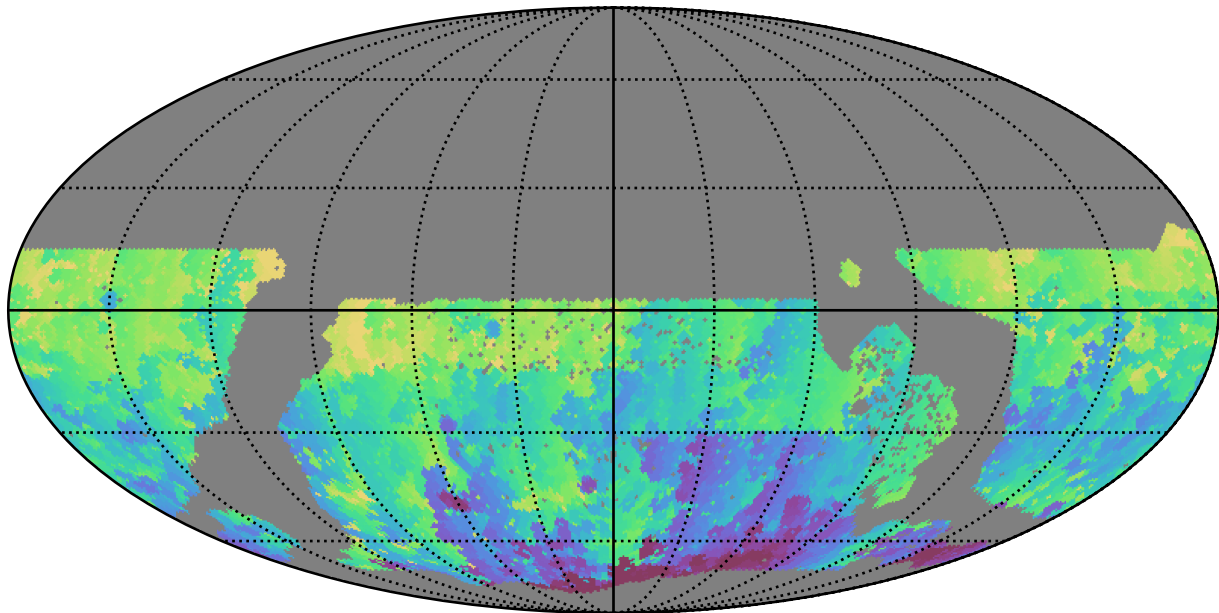
ddf_acor_sf20_lsf40_lsr50_v3.4_10yrs WFD u band: Min HA
