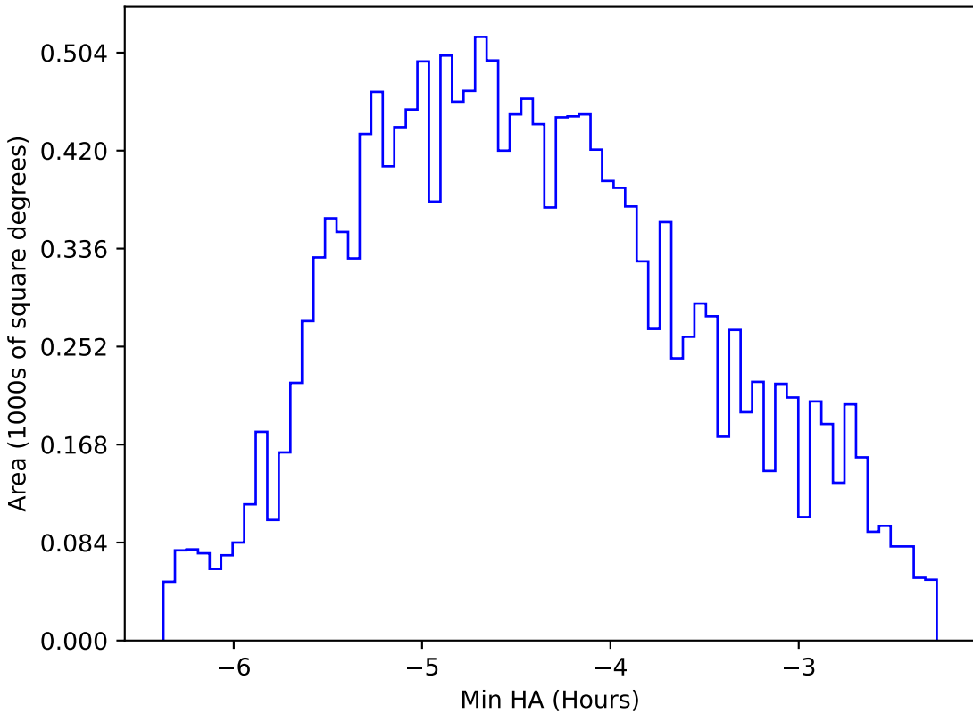
ddf_acor_sf20_lsf40_lsr50_v3.4_10yrs WFD r band: Min HA
