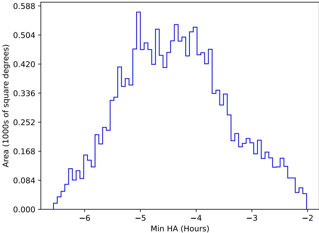
ddf_acor_sf20_Isf40_Isr50_v3.4_10yrs WFD i band: Min HA
