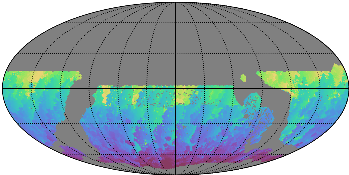
ddf_acor_sf20_lsf40_lsr50_v3.4_10yrs WFD g band: Min HA
