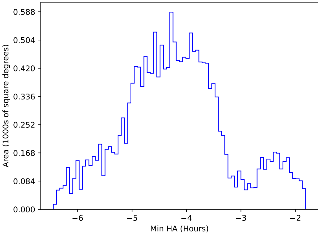
ddf_acor_sf20_lsf40_lsr50_v3.4_10yrs WFD g band: Min HA
