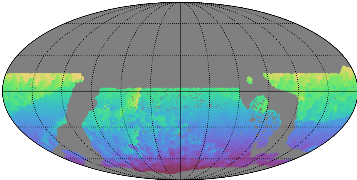
ddf_acor_sf20_lsf40_lsr50_v3.4_10yrs WFD all bands: Min HA
