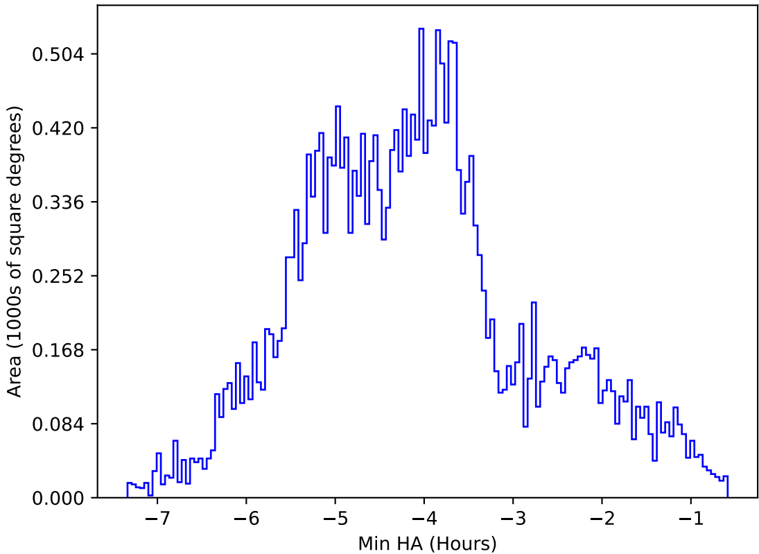
ddf_acor_sf20_lsf40_lsr50_v3.4_10yrs All sky z band: Min HA
