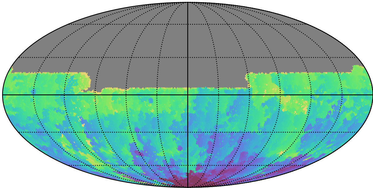
ddf_acor_sf20_lsf40_lsr50_v3.4_10yrs All sky u band: Min HA
