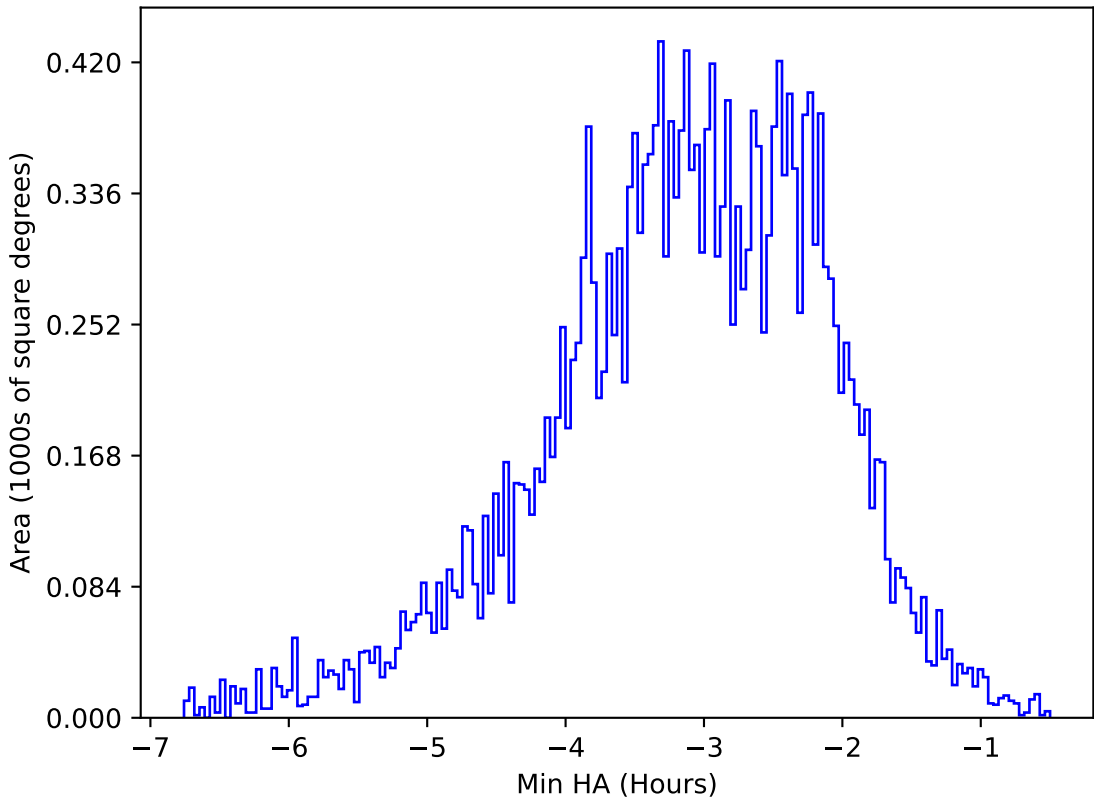
ddf_acor_sf20_lsf40_lsr50_v3.4_10yrs All sky u band: Min HA
