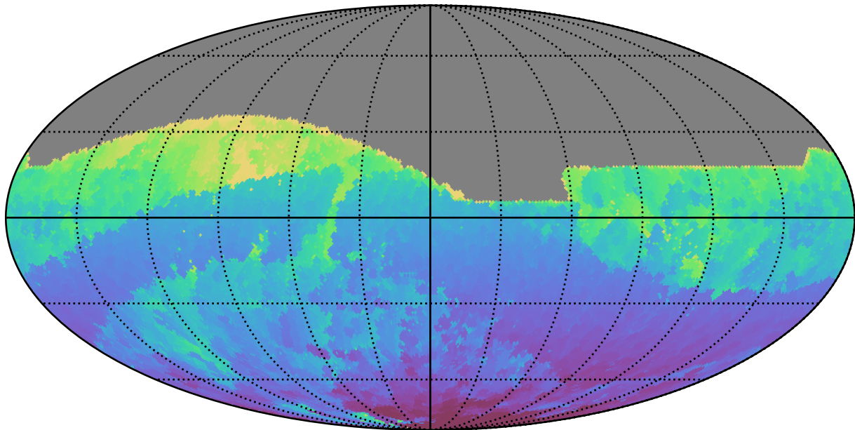
ddf_acor_sf20_lsf40_lsr50_v3.4_10yrs All sky r band: Min HA
