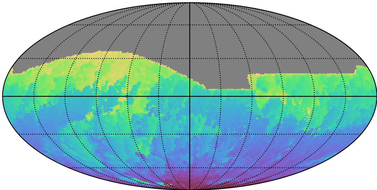
ddf_acor_sf20_lsf40_lsr50_v3.4_10yrs All sky i band: Min HA
