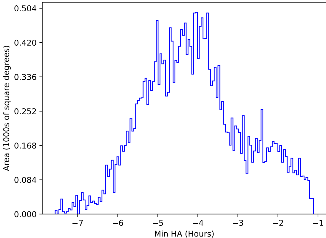
ddf_acor_sf20_ls40_lsr50_v3.4_10yrs All sky i band: Min HA
