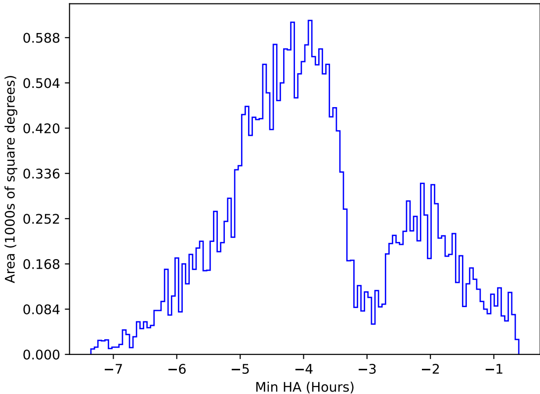
ddf_acor_sf20_lsf40_lsr50_v3.4_10yrs All sky g band: Min HA
