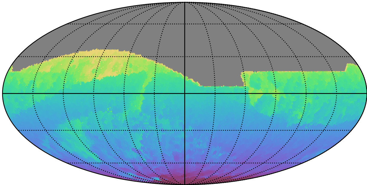
ddf_acor_sf20_lsf40_lsr50_v3.4_10yrs All sky all bands: Min HA
