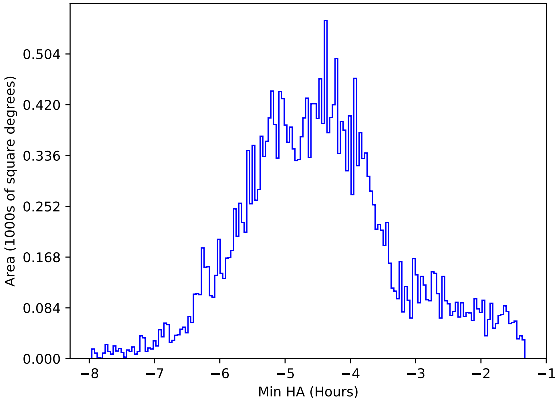
ddf_acor_sf20_lsf40_lsr50_v3.4_10yrs All sky all bands: Min HA
