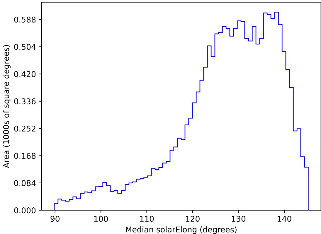
ddf_acor_sf20_lsf40_lsr50_v3.4_10yrs WFD z band: Median solarElong
