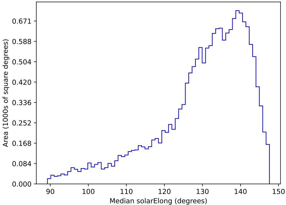
ddf_acor_sf20_lsf40_lsr50_v3.4_10yrs WFD y band: Median solarElong
