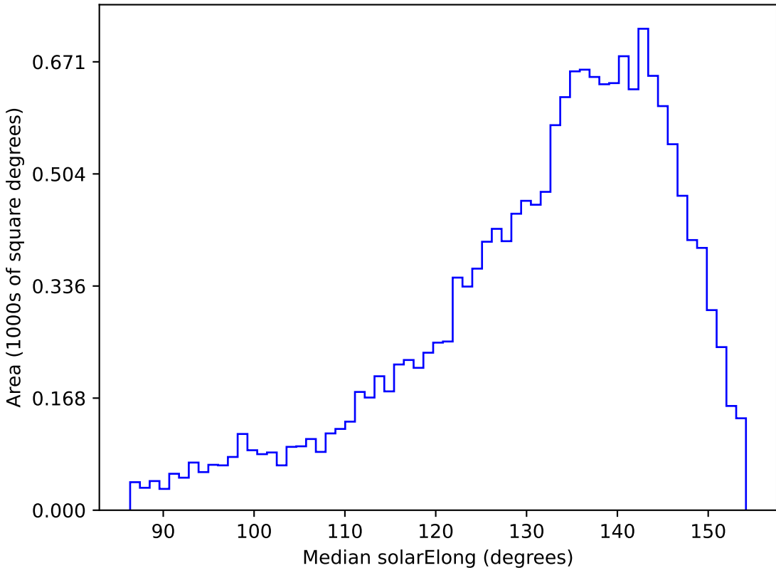
ddf_acor_sf20_lsf40_lsr50_v3.4_10yrs WFD u band: Median solarElong
