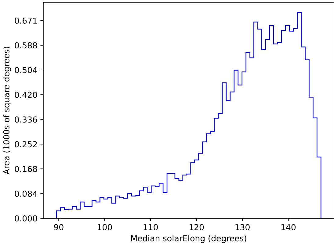
ddf_acor_sf20_lsf40_lsr50_v3.4_10yrs WFD r band: Median solarElong
