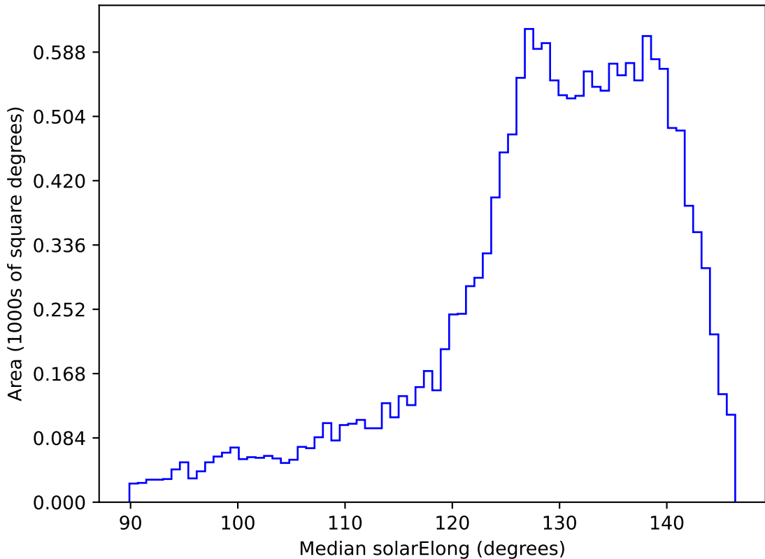
ddf_acor_sf20_lsf40_lsr50_v3.4_10yrs WFD i band: Median solarElong
