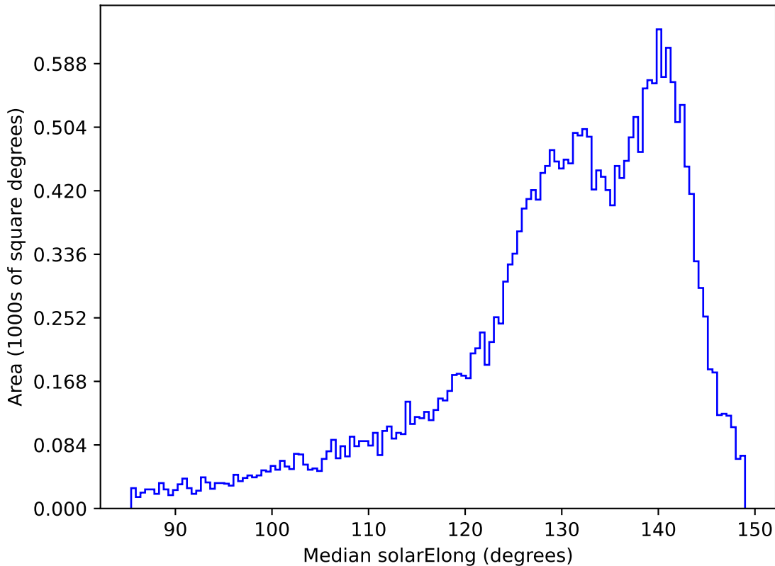
ddf_acor_sf20_lsf40_lsr50_v3.4_10yrs All sky all bands: Median solarElong
