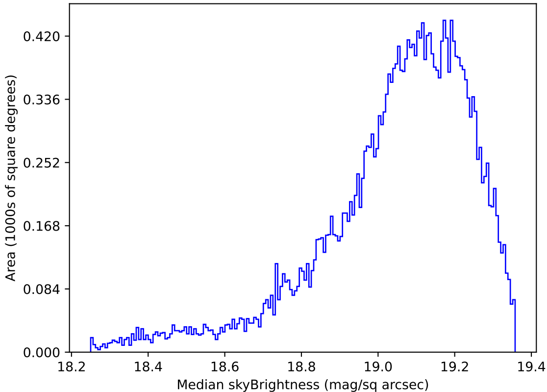
ddf_acor_sf20_lsf40_lsr50_v3.4_10yrs Yr 1 z band: Median skyBrightness
