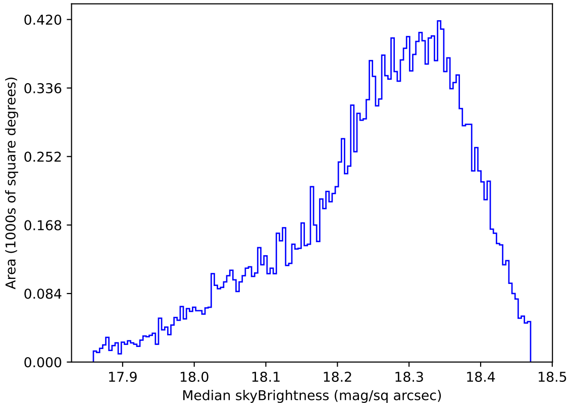
ddf_acor_sf20_lsf40_lsr50_v3.4_10yrs Yr 1 y band: Median skyBrightness
