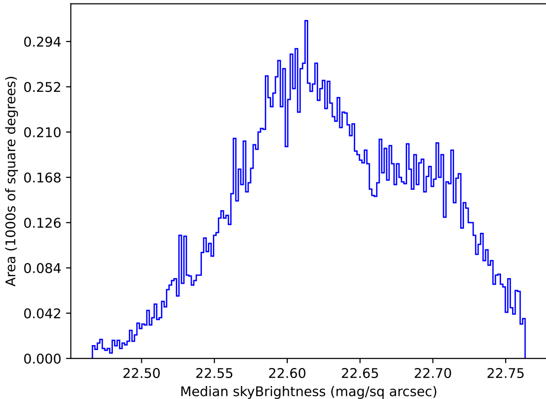
ddf_acor_sf20_lsf40_lsr50_v3.4_10yrs Yr 1 u band: Median skyBrightness
