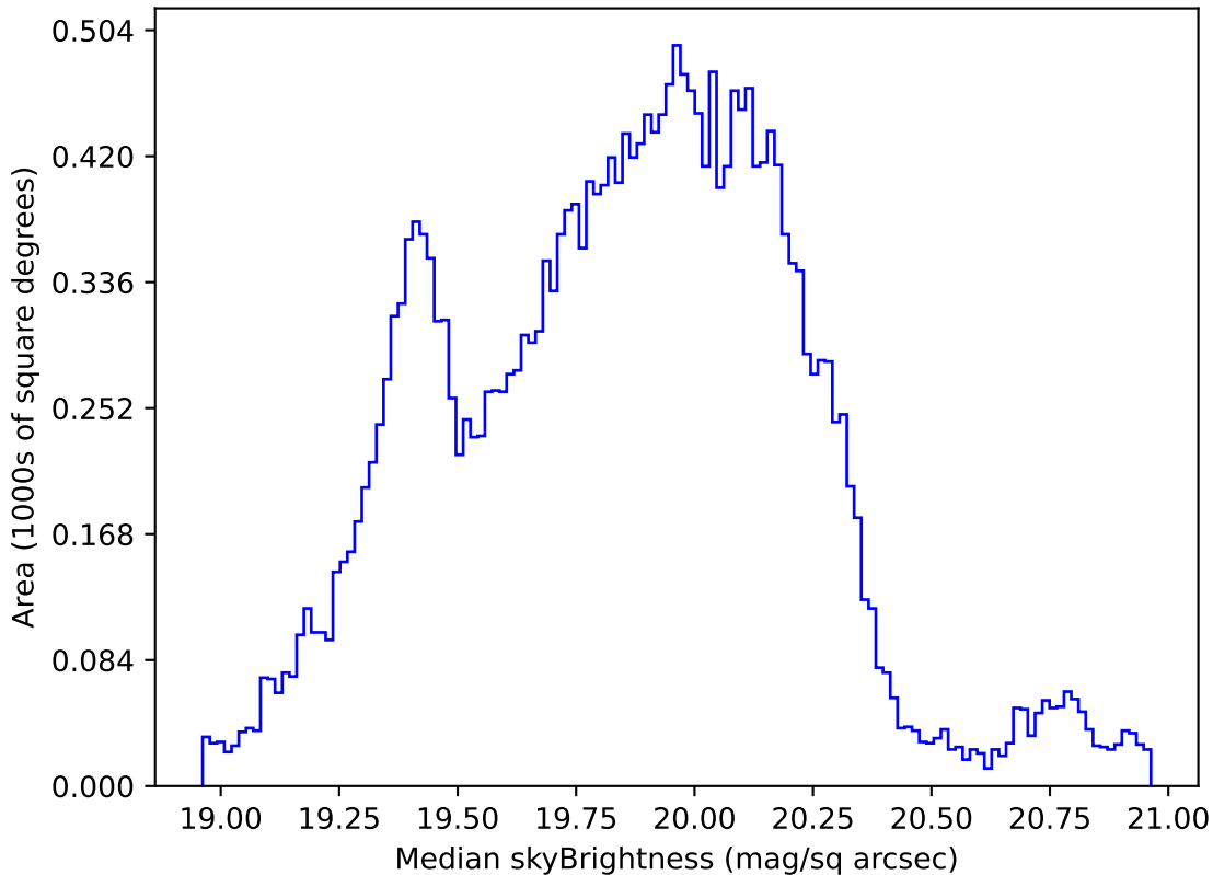
ddf_acor_sf20_lsf40_lsr50_v3.4_10yrs Yr 1 all bands: Median skyBrightness
