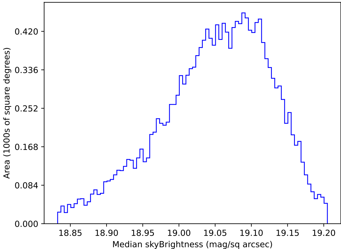
ddf_acor_sf20_lsf40_lsr50_v3.4_10yrs WFD z band: Median skyBrightness
