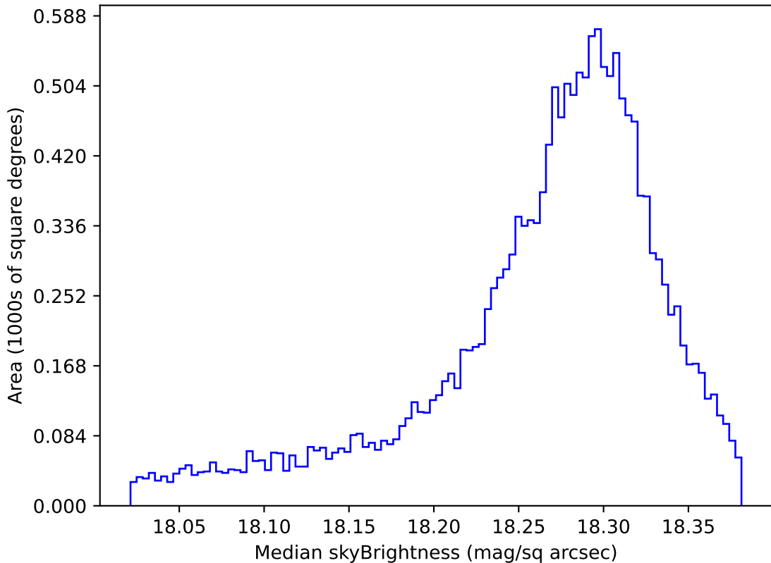
ddf_acor_sf20_lsf40_lsr50_v3.4_10yrs WFD y band: Median skyBrightness
