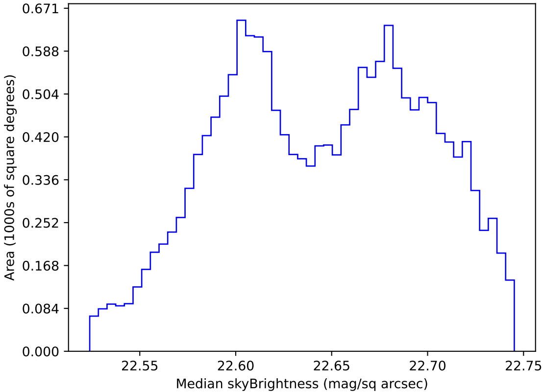
ddf_acor_sf20_lsf40_lsr50_v3.4_10yrs WFD u band: Median skyBrightness
