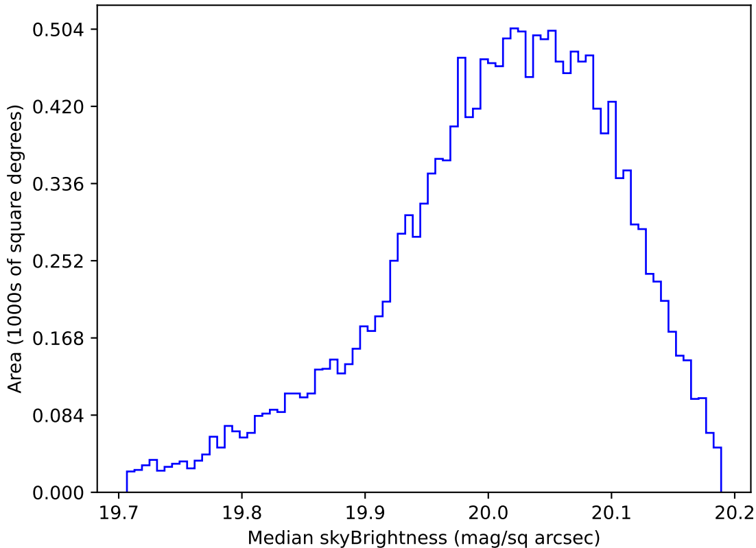
ddf_acor_sf20_lsf40_lsr50_v3.4_10yrs WFD i band: Median skyBrightness
