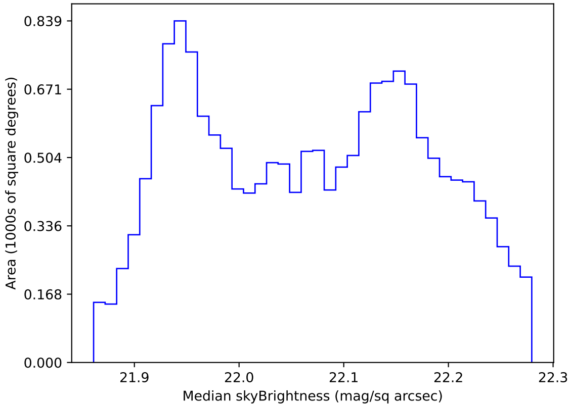
ddf_acor_sf20_lsf40_lsr50_v3.4_10yrs WFD g band: Median skyBrightness
