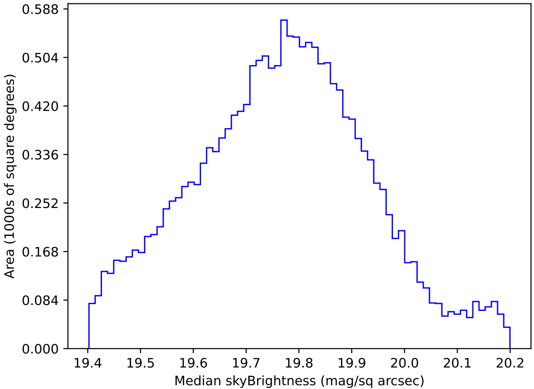
ddf_acor_sf20_lsf40_lsr50_v3.4_10yrs WFD all bands: Median skyBrightness
