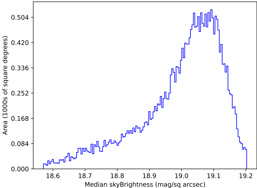
ddf_acor_sf20_lsf40_lsr50_v3.4_10yrs All sky z band: Median skyBrightness
