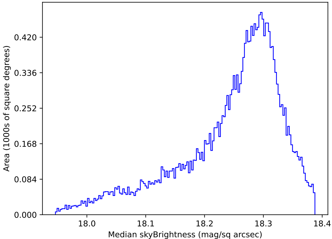
ddf_acor_sf20_lsf40_lsr50_v3.4_10yrs All sky y band: Median skyBrightness
