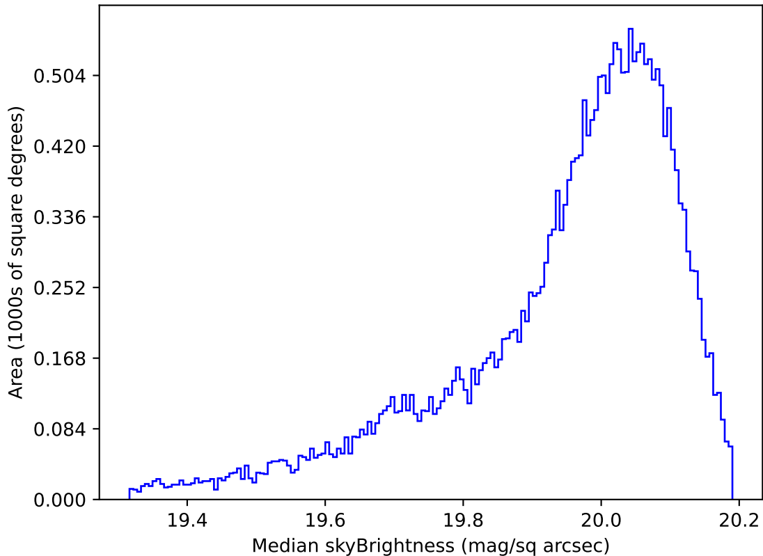
ddf_acor_sf20_lsf40_lsr50_v3.4_10yrs All sky i band: Median skyBrightness
