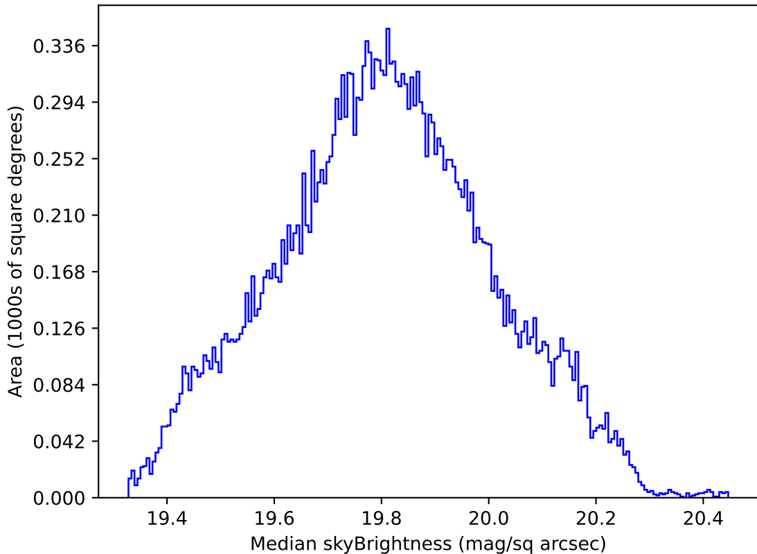
ddf_acor_sf20_lsf40_lsr50_v3.4_10yrs All sky all bands: Median skyBrightness
