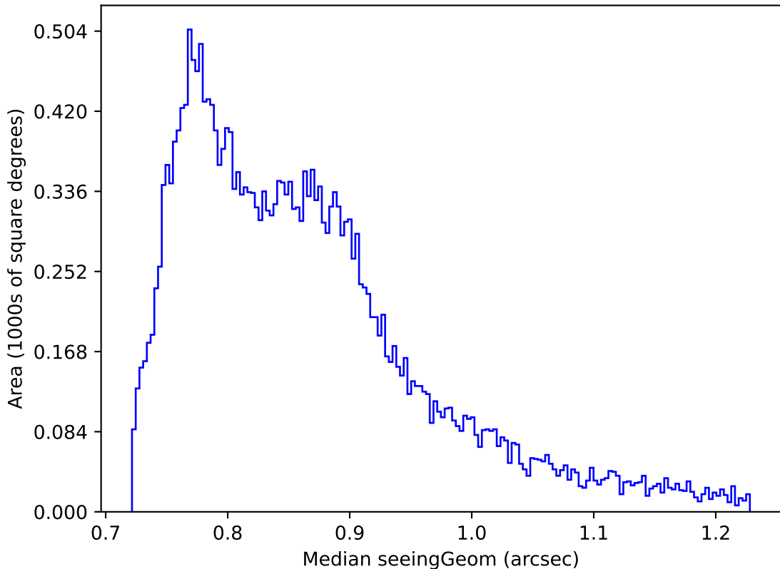
ddf_acor_sf20_lsf40_lsr50_v3.4_10yrs Yr 1 all bands: Median seeingGeom
