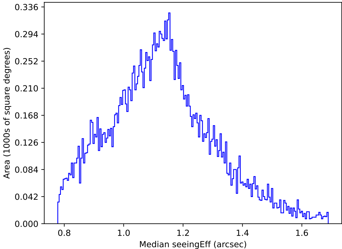
ddf_acor_sf20_lsf40_lsr50_v3.4_10yrs Yr 1 u band: Median seeingEff
