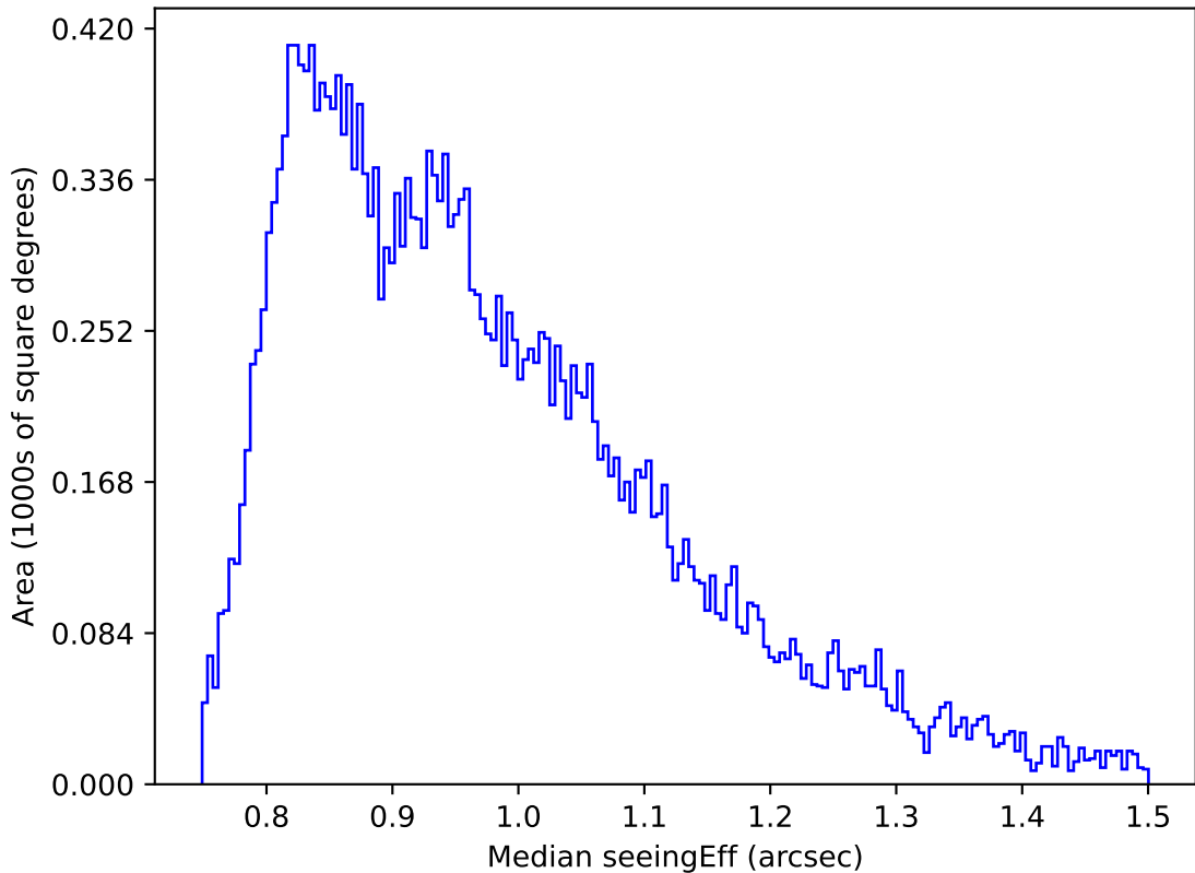
ddf_acor_sf20_lsf40_lsr50_v3.4_10yrs Yr 1 r band: Median seeingEff
