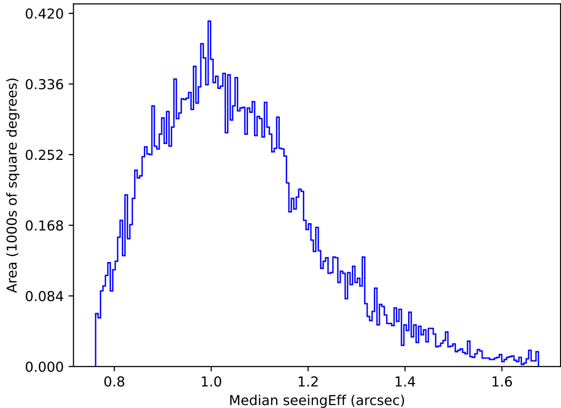
ddf_acor_sf20_lsf40_lsr50_v3.4_10yrs Yr 1 g band: Median seeingEff
