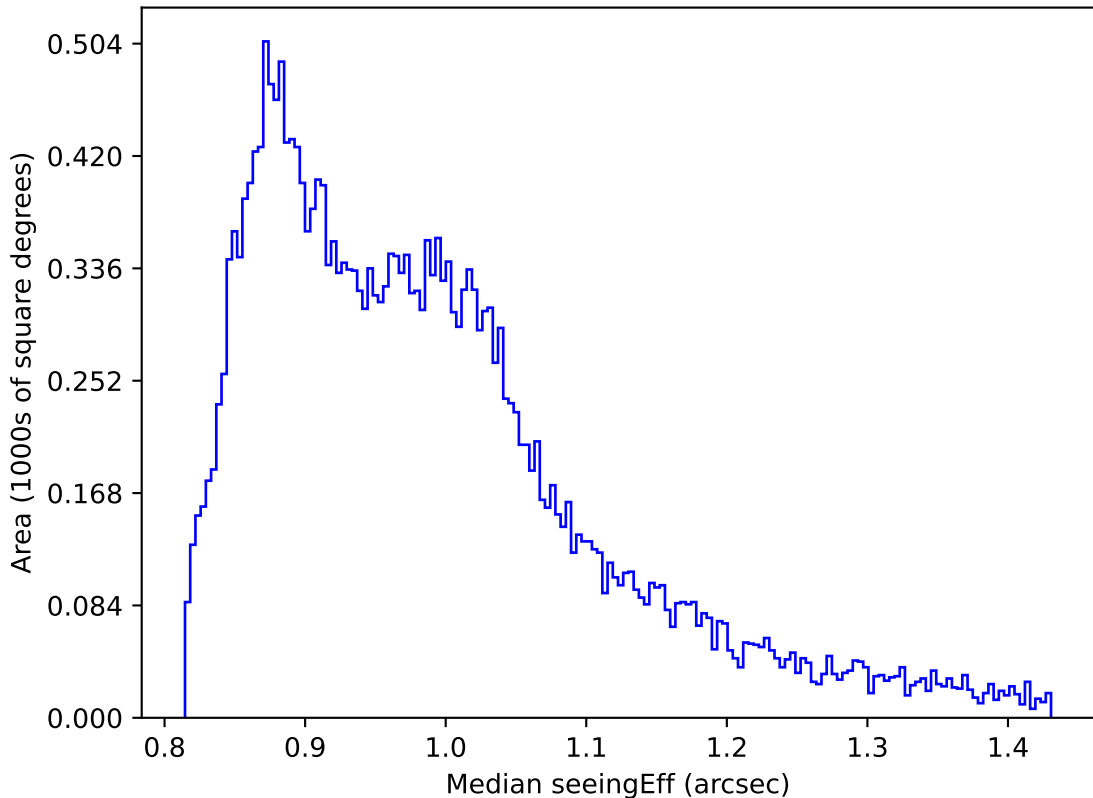
ddf_acor_sf20_lsf40_lsr50_v3.4_10yrs Yr 1 all bands: Median seeingEff
