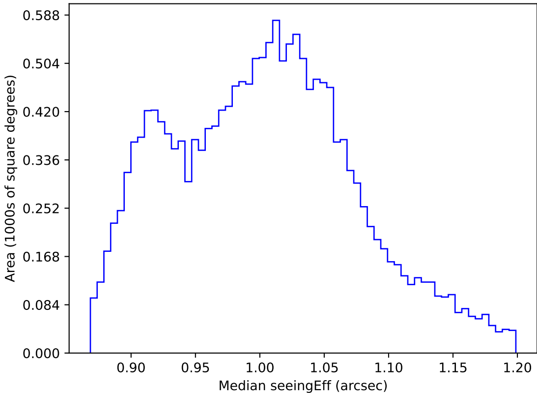
ddf_acor_sf20_lsf40_lsr50_v3.4_10yrs WFD z band: Median seeingEff
